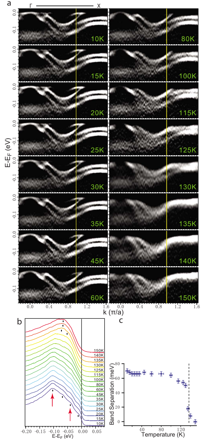
FIG. 5. (Color online) Temperature evolution of BaFe 2 As 2 band dispersions across the T_{SDW} . (a) Second derivatives of spectra along the \Gamma -X high symmetry cut showing the temperature evolution of band dispersions across T_{SDW} . (b) Temperature dependence of a single EDC [momentum position marked by the yellow lines in (a)] across T_{SDW} . The peak positions mark the band binding-energy positions at this momentum. (c) Separation of the two bands in energy [marked by arrows in (b)] as a function of temperature across T_{SDW}=137 K.
