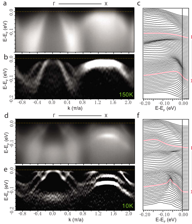
FIG. 4. (Color online) Contrast of BaFe 2 As 2 band dispersions across the T_{SDW} . (a) Raw spectra image along the \Gamma -X high symmetry cut above T_{SDW} ( T=150 K). (b) Second derivative image of (a). (c) EDCs of the cut in (a). (d)–(f) same as in (a)–(c) but taken below T_{SDW} ( T=10 K).
